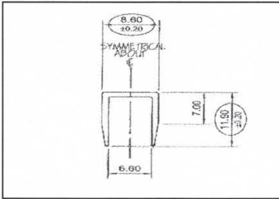
T012 U Trimming 6.60mm
