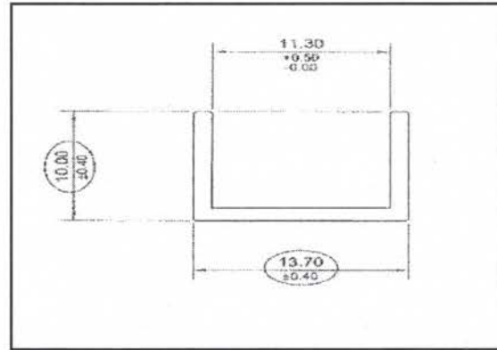
T01201 U Trimming 11.30mm
