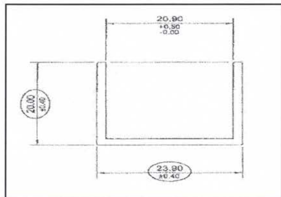
T012F U Trimming 20.90mm
