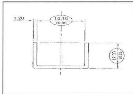
T012D U Trimming 15.10mm
