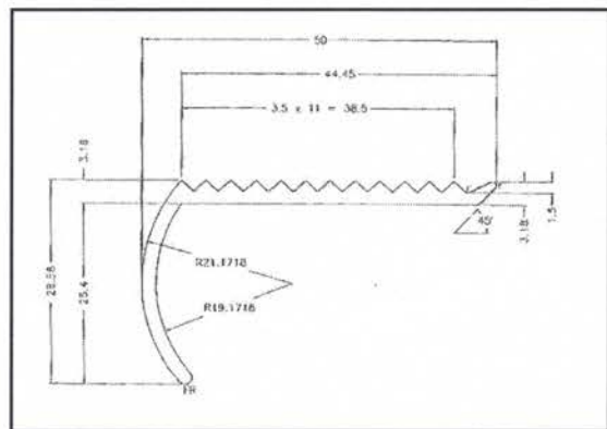
T002 Stair Case Nose Strip
